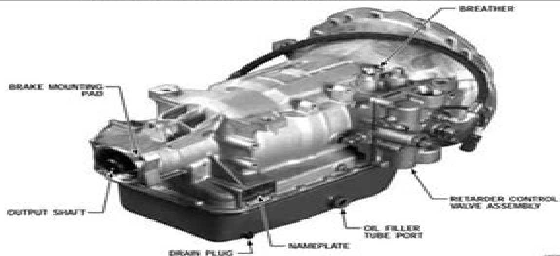
Figure 1-2. AT 545R Automatic Transmission — Right-Rear View
