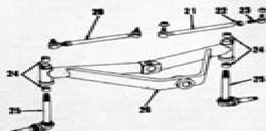
Fig. 7—Heavy duty non-adjustable front axle available for International 544 and 656 tractors. Refer to Fig. 8 for balance of components.
