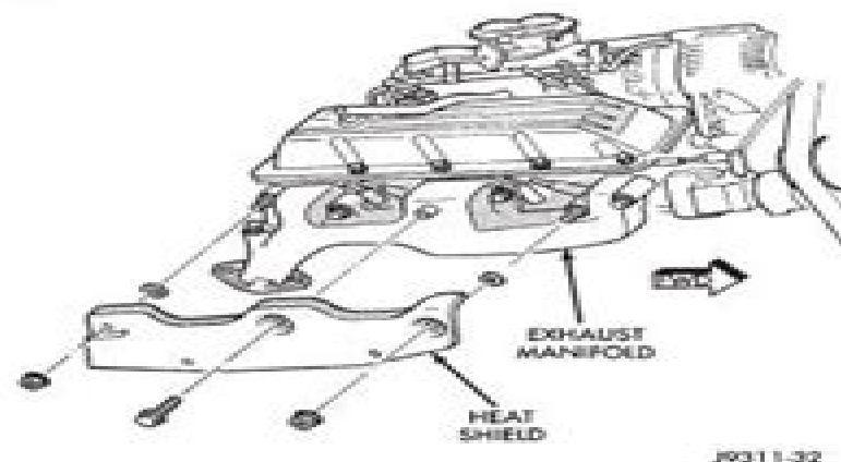
Fig. 12 Exhaust Manifold Heat Shields (Left Shield Shown)
