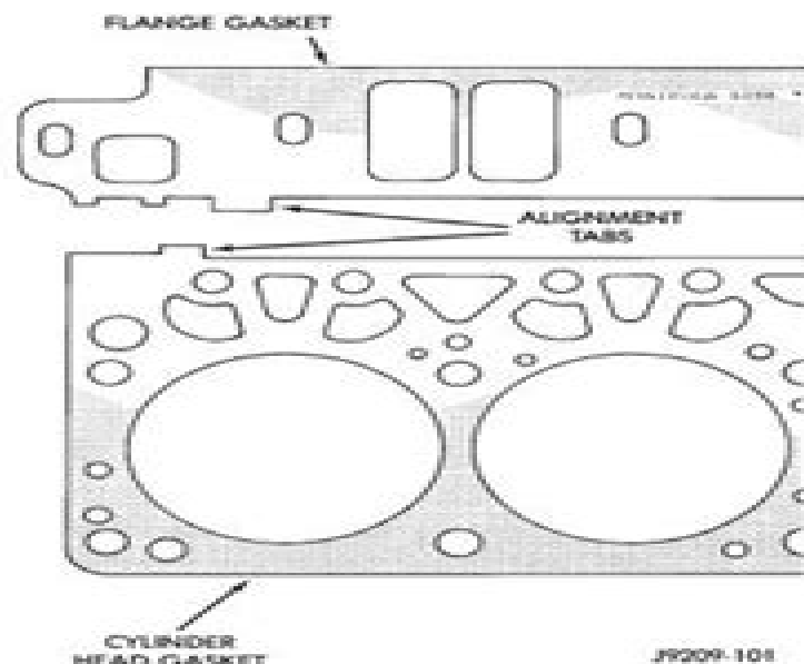
Fig. 10 Intake Manifold Flange Gasket Alignment
