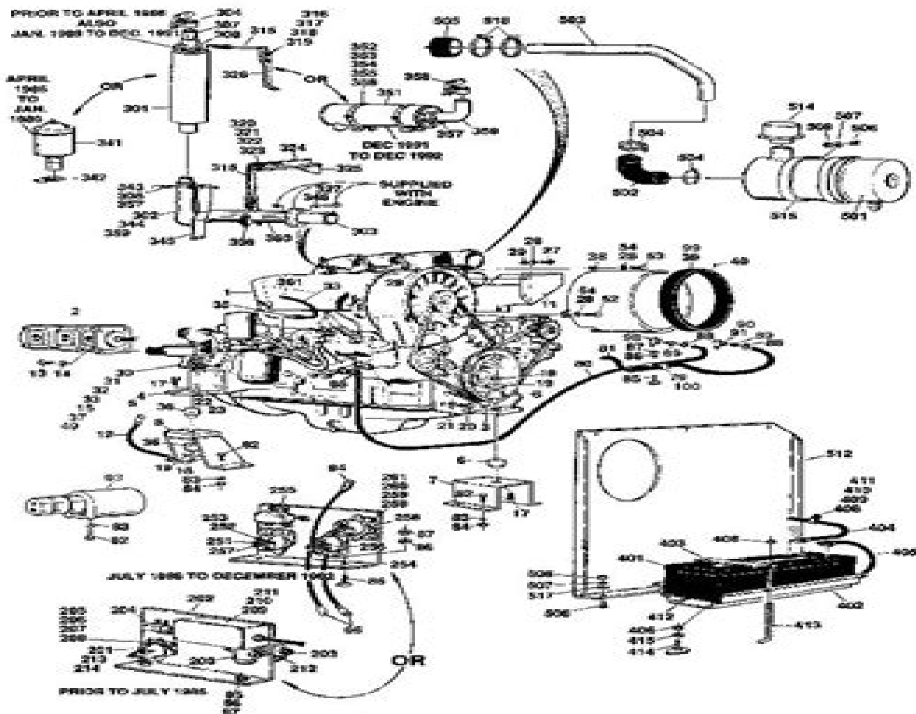
FIGURE 2-24. DEUTZ ENGINE INSTALLATION WITHOUT NOISE REDUCTION (BUILT PRIOR TO DECEMBER 1992)
