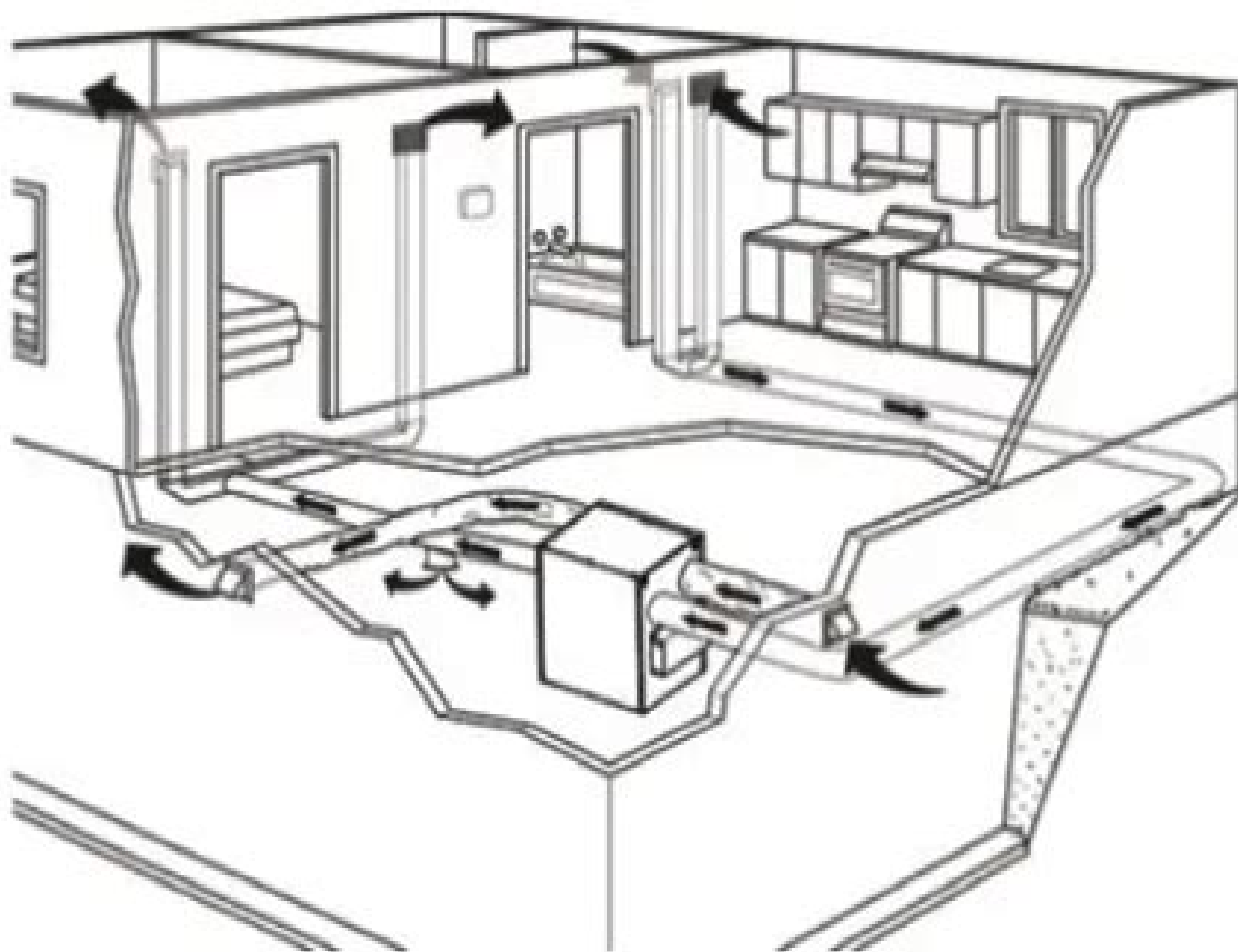
Fig. 5 – Fully Ducted System
