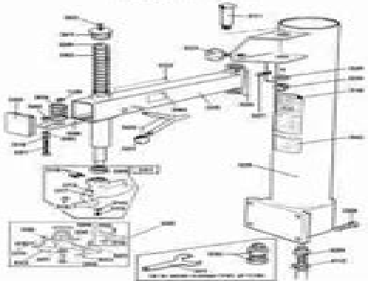
Figure 7 Vertical Post
