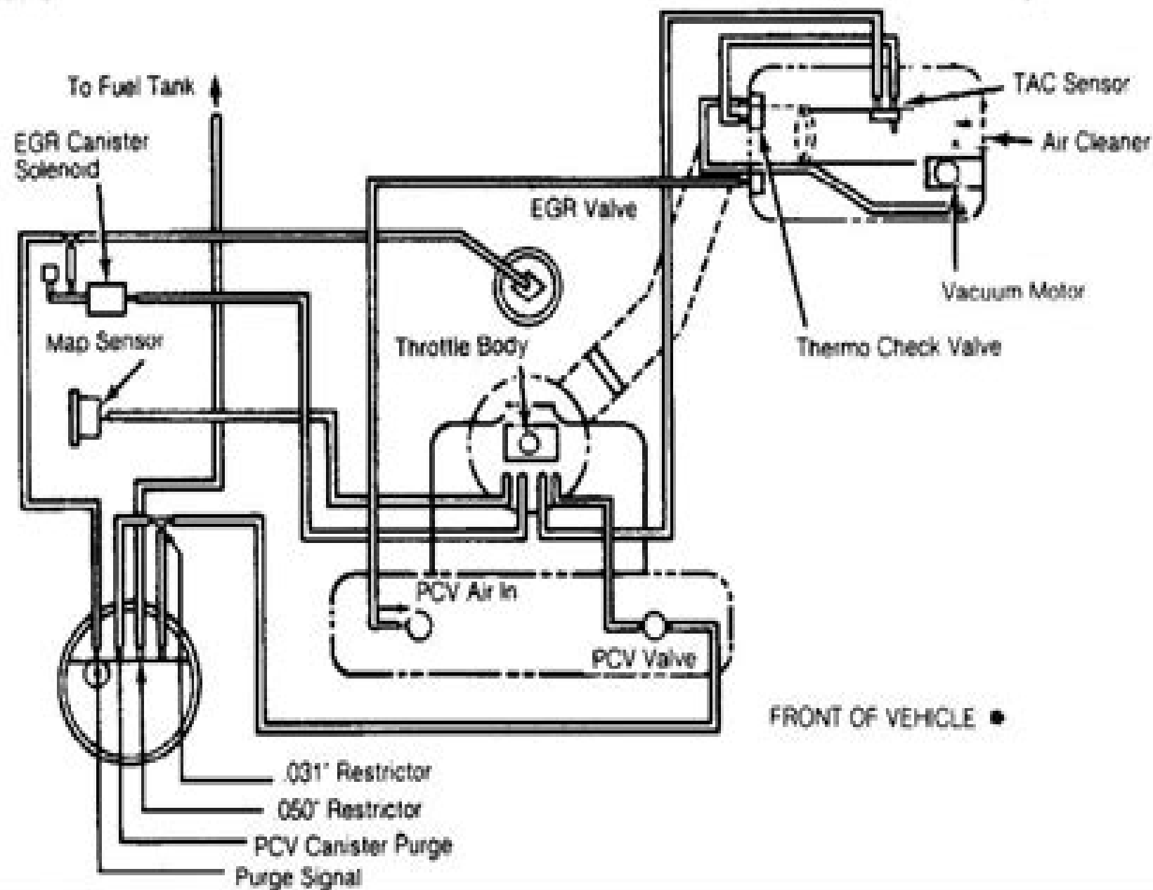
Fig. 1: 2.5L 4-Cylinder
