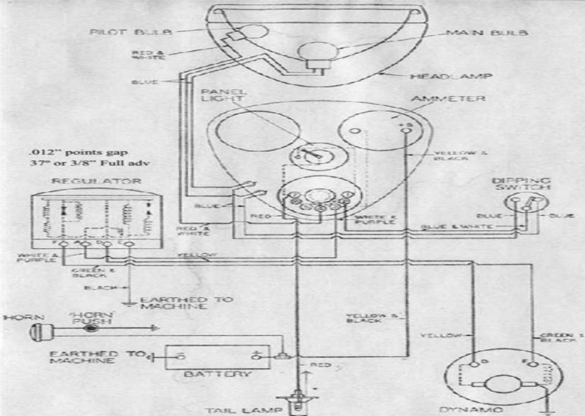
FIG. 36. WIRING DIAGRAM FOR 1937-9 LUCAS "MAGDYN0" LIGHTING EQUIPMENT WITH AUTOMATIC VOLTAGE CONTROL AND INSTRUMENT PANEL
