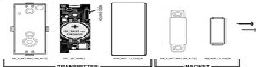
Fig. 1. GEM-TRANSLP Component Parts
