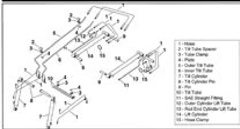
Fig. 9-30 Exploded view of LiTTit Self-Leveling Hydraulics - Lift Arm - SX Models.
