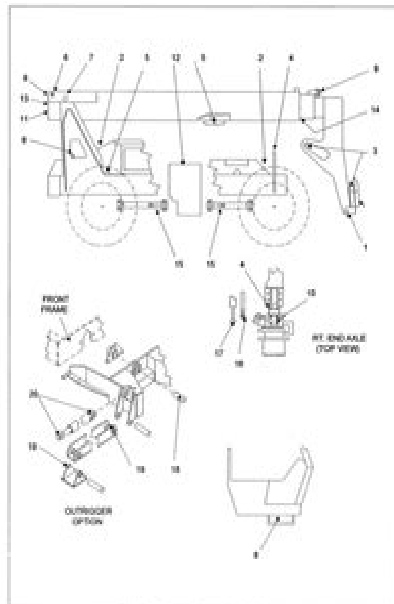
Fig. 12 - Grease Fittings, Basic Machine & Outriggers
