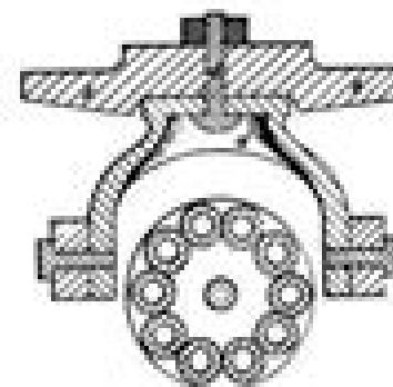
FIG. 5. SECTION THROUGH BARREL, BREECH AND MUZZLE BLOCK.
