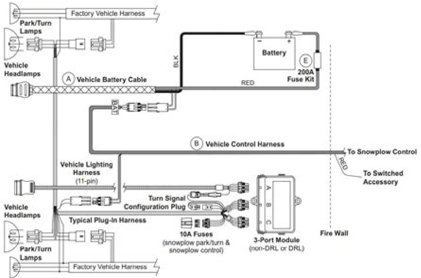
Vehicle-Side Harness Diagram
