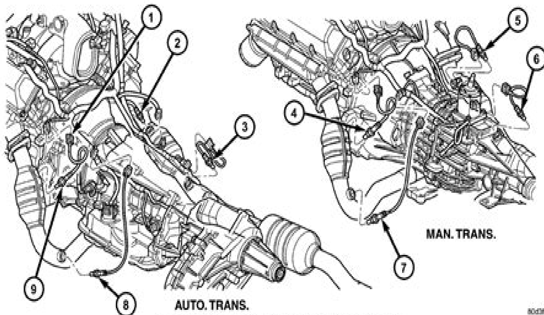
Fig. 32 O2S LOCATION - 3.7L/4.7L CALIFORNIA
