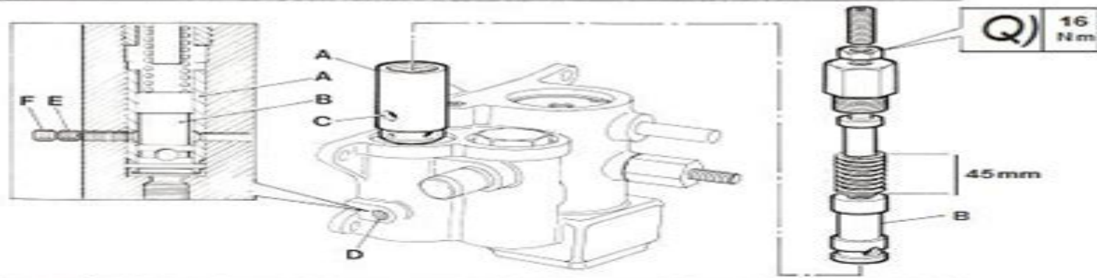
Servo-Valve
