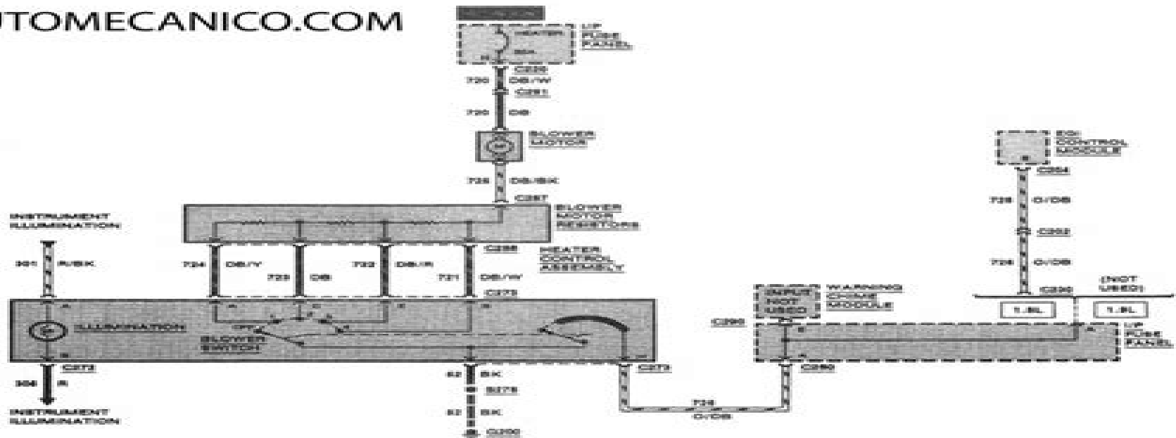
Heater wiring diagram - 1991 through 1996 models
