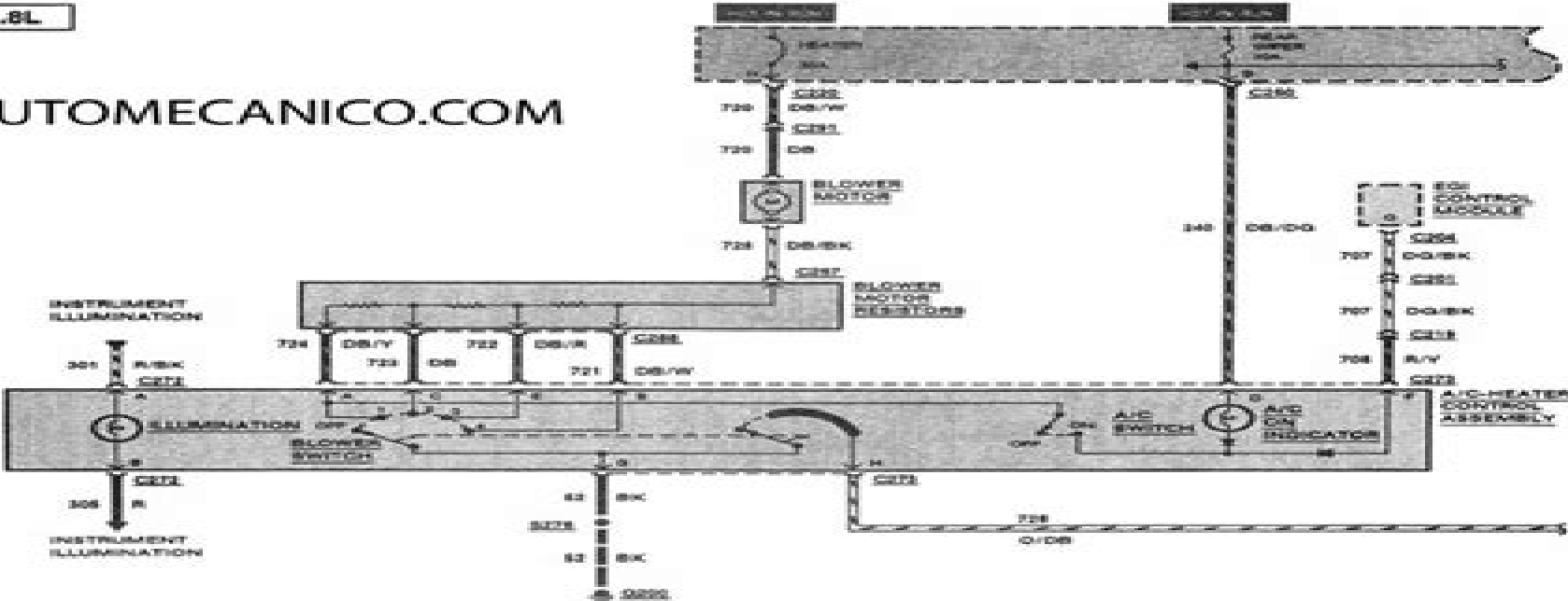
Heater/air conditioner wiring diagram, 1.8L engine - 1991 through 1996 models (part 1 of 2)
