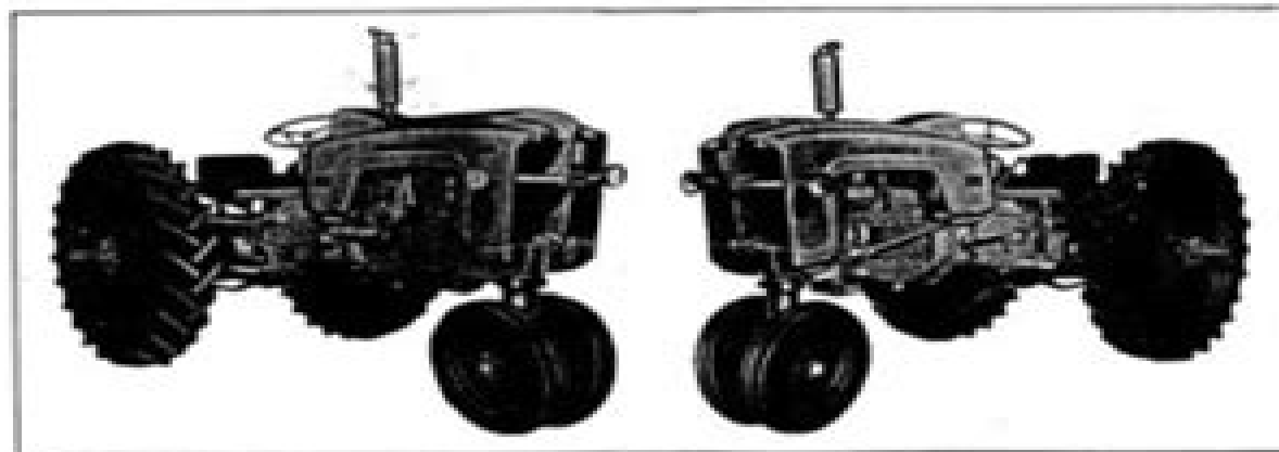
Fig. 2. Right and left views of a 445 Universal Tractor with the Type D (dual wheels) front wheel assembly installed.
