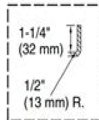
Integral Flange Detail
