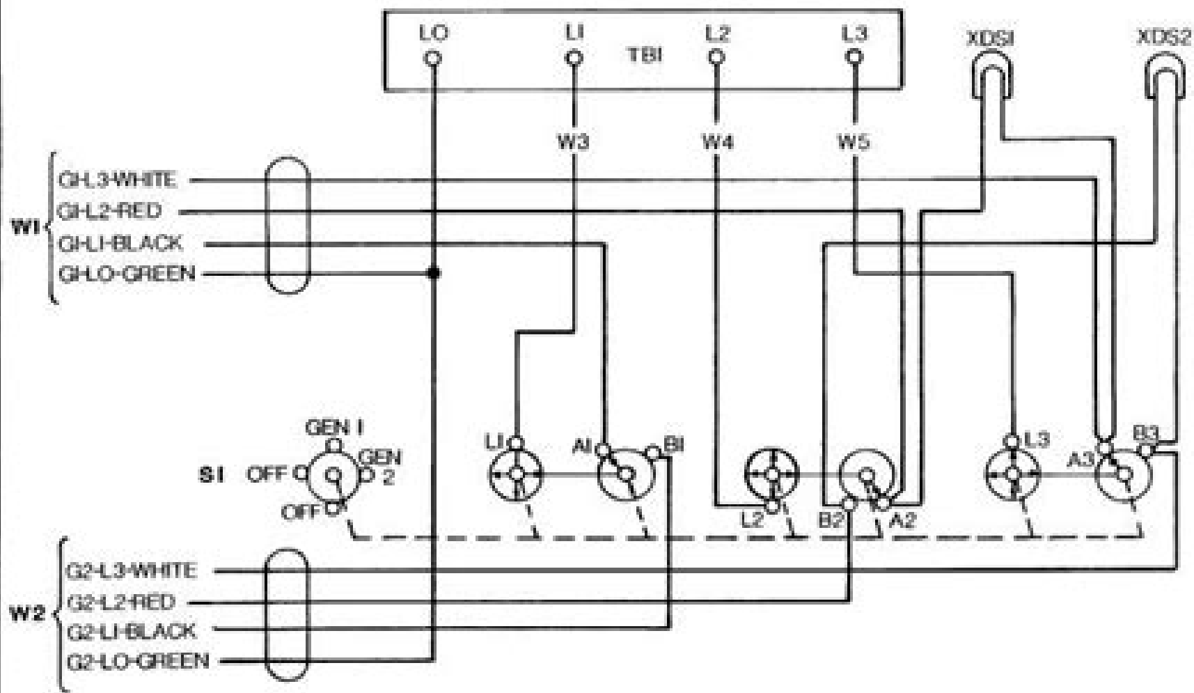
TRANSFER SWITCH WIRING DIAGRAM
