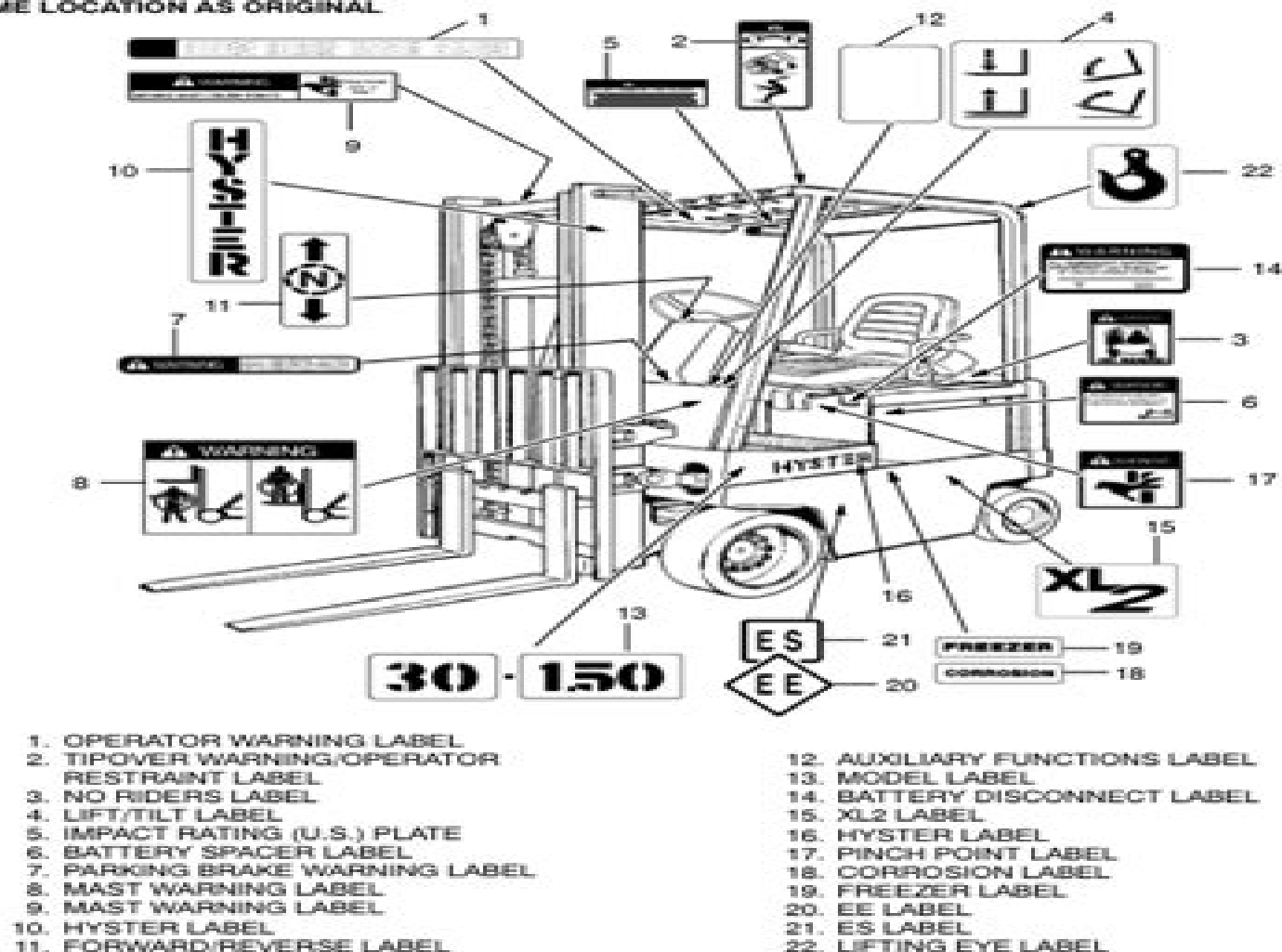
FIGURE 15. LABEL POSITIONS, E/JL25-1.75XL (E25-35XL)
