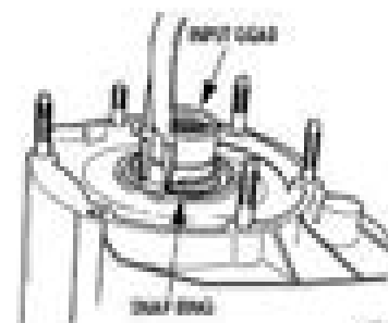
Figure 6-188 Input gear drag ring removal
