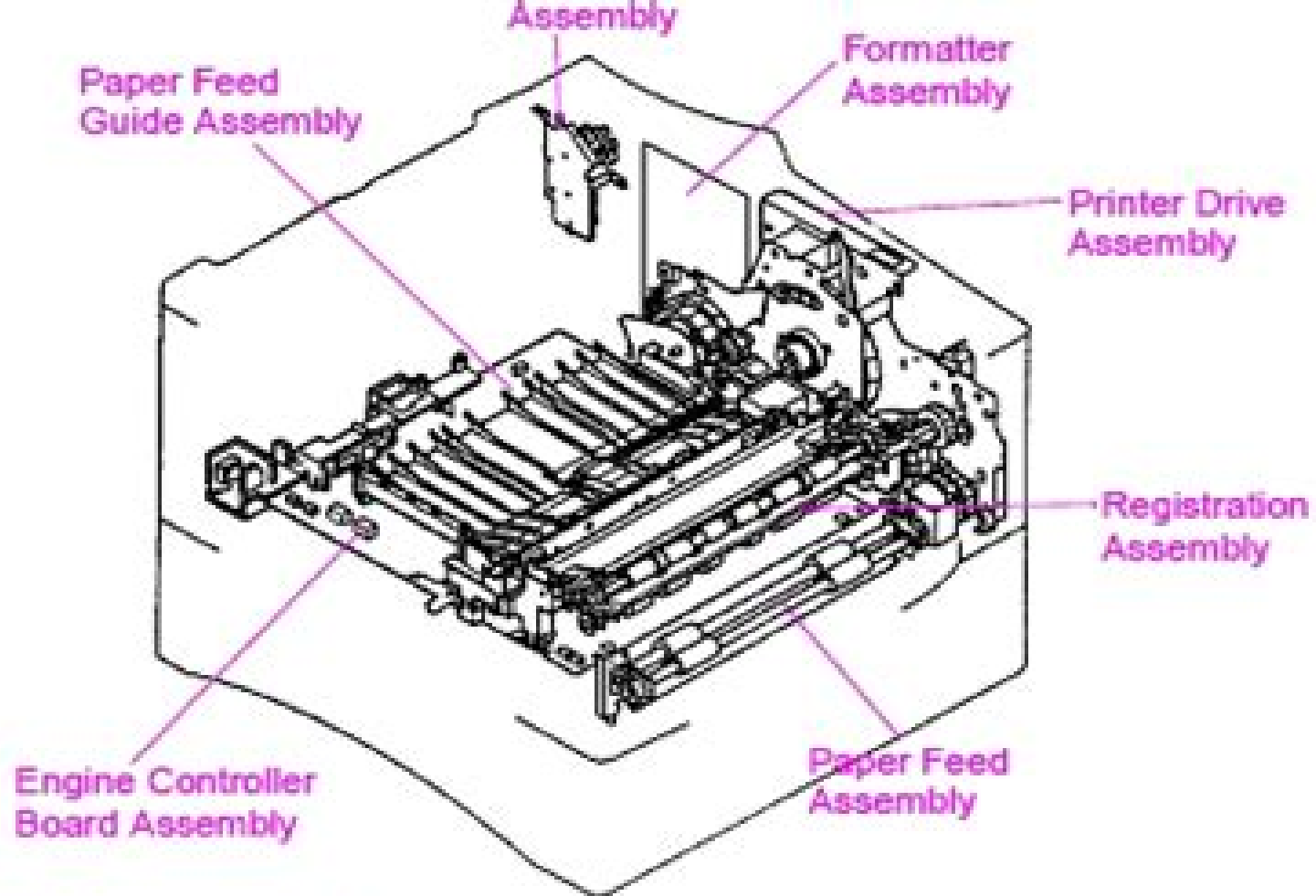
Figure 8-1 Assembly Location Diagram
