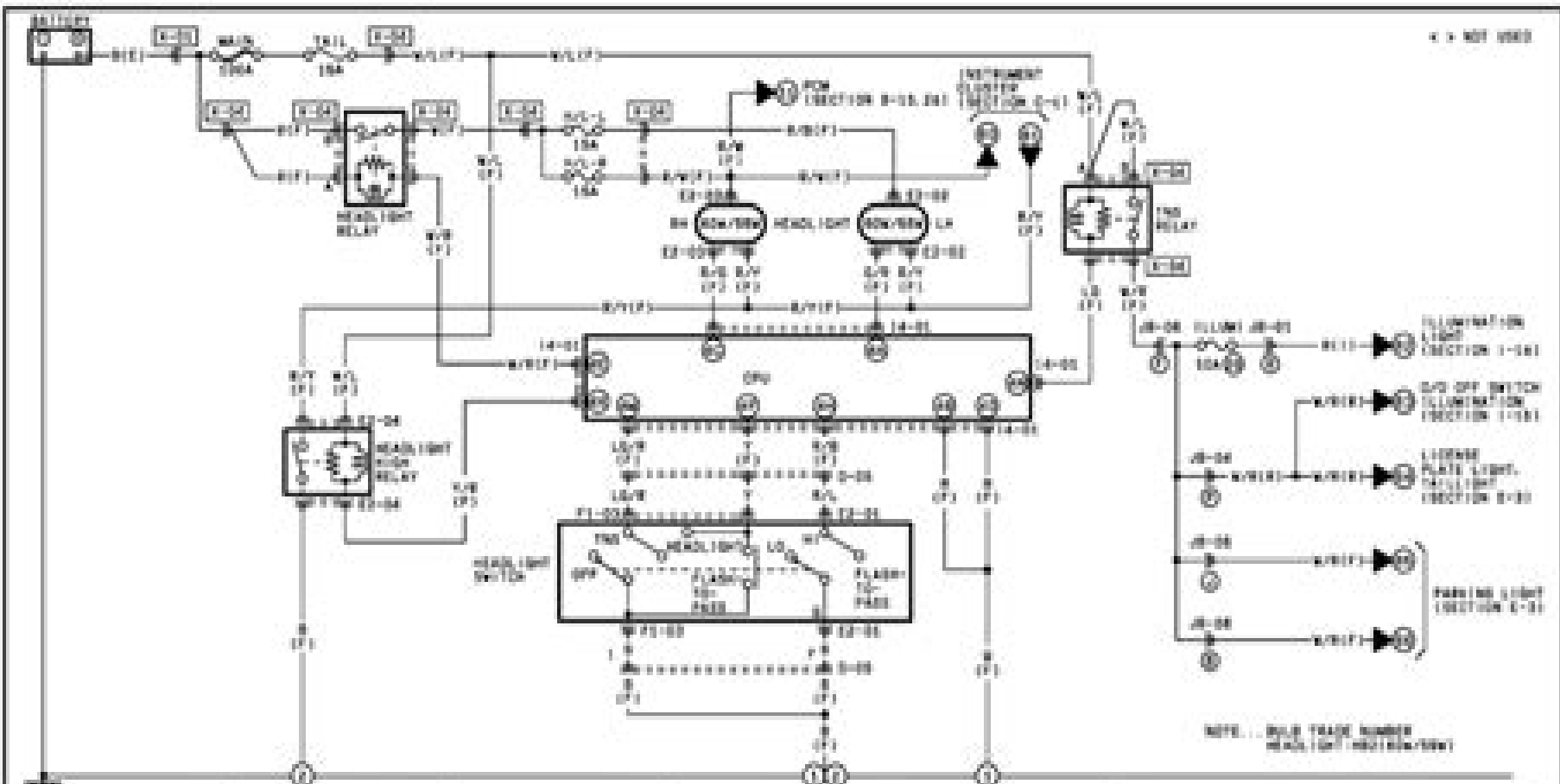
F1-01 HEADLIGHT SWITCH (SHORT CORN)
