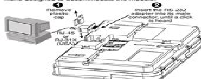
Figure 3.4 - Connecting the PowerMax+ to a Computer
