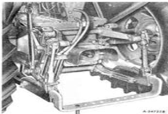
Illustr. 1 Two-Point Fast-Hitch with Traction Control.
