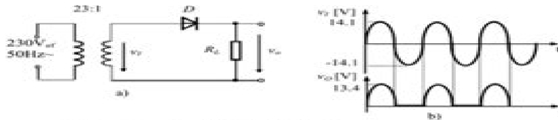
Fig. 1. Half-wave rectifier a) Circuit; b) Waveforms;
