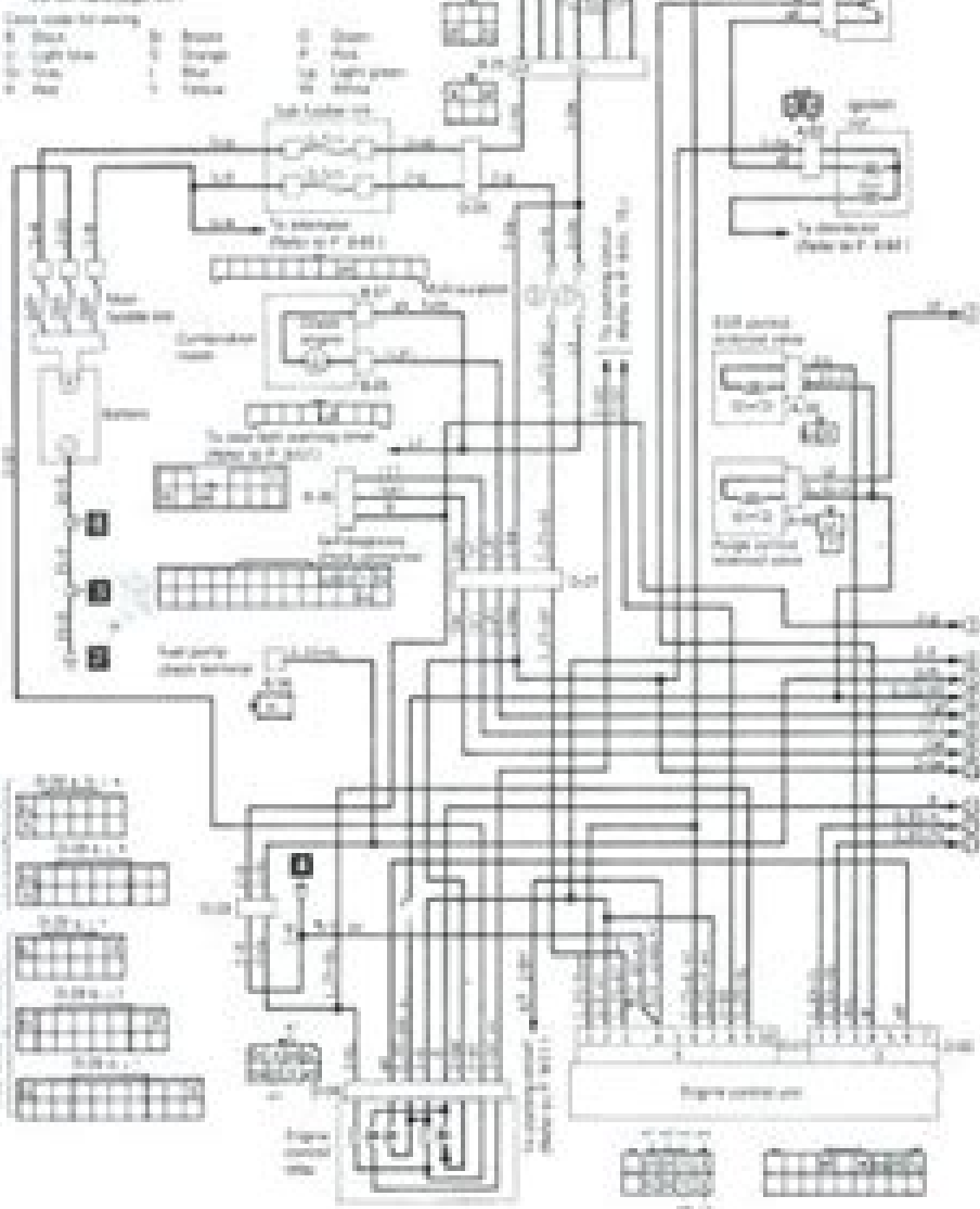
20.11a Fuel injection circuit (2.4L engine - 1 of 2)
