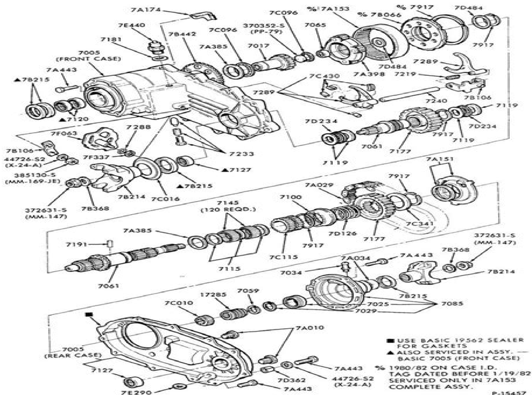
TRANSFER CASE — NEW PROCESS NP 208 — PART TIME 1980/86 F—U 150/350
