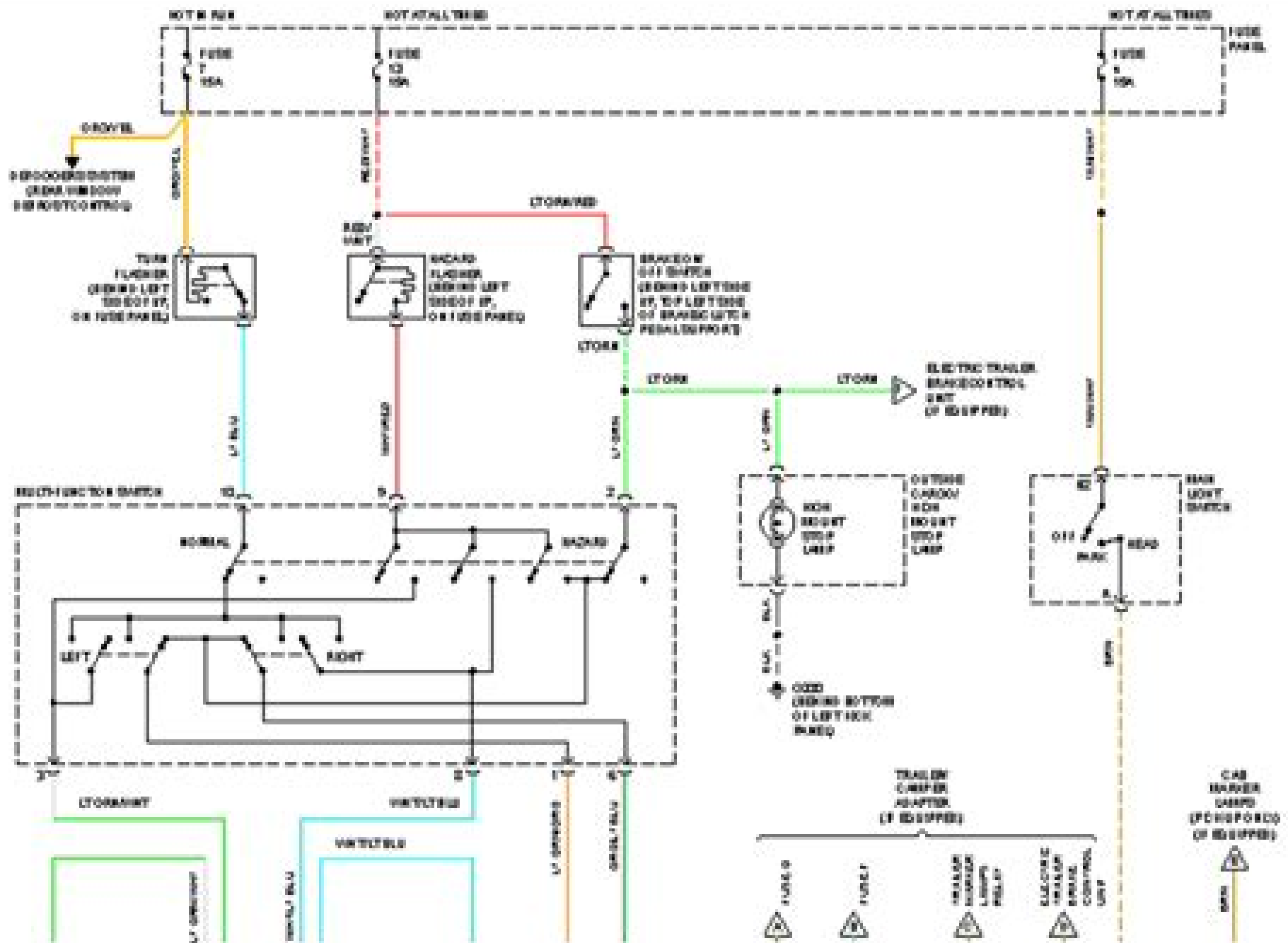
1994 Ford Pickup F150-Fig. 32: Exterior Lamps Circuit (1 of 2)
