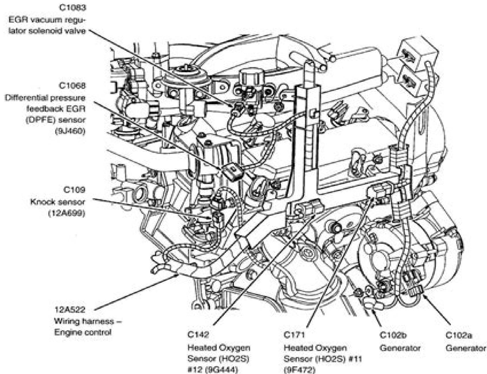
engine, rear, Duratec engine
