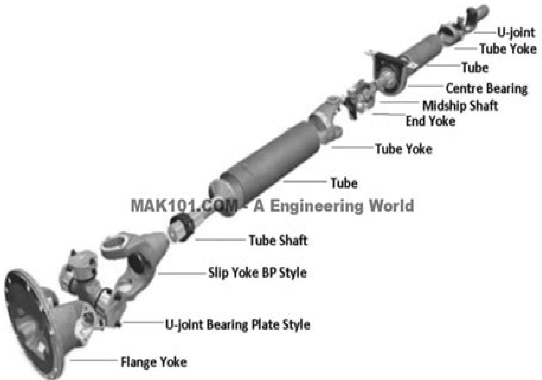
Parts of Propeller Shaft
