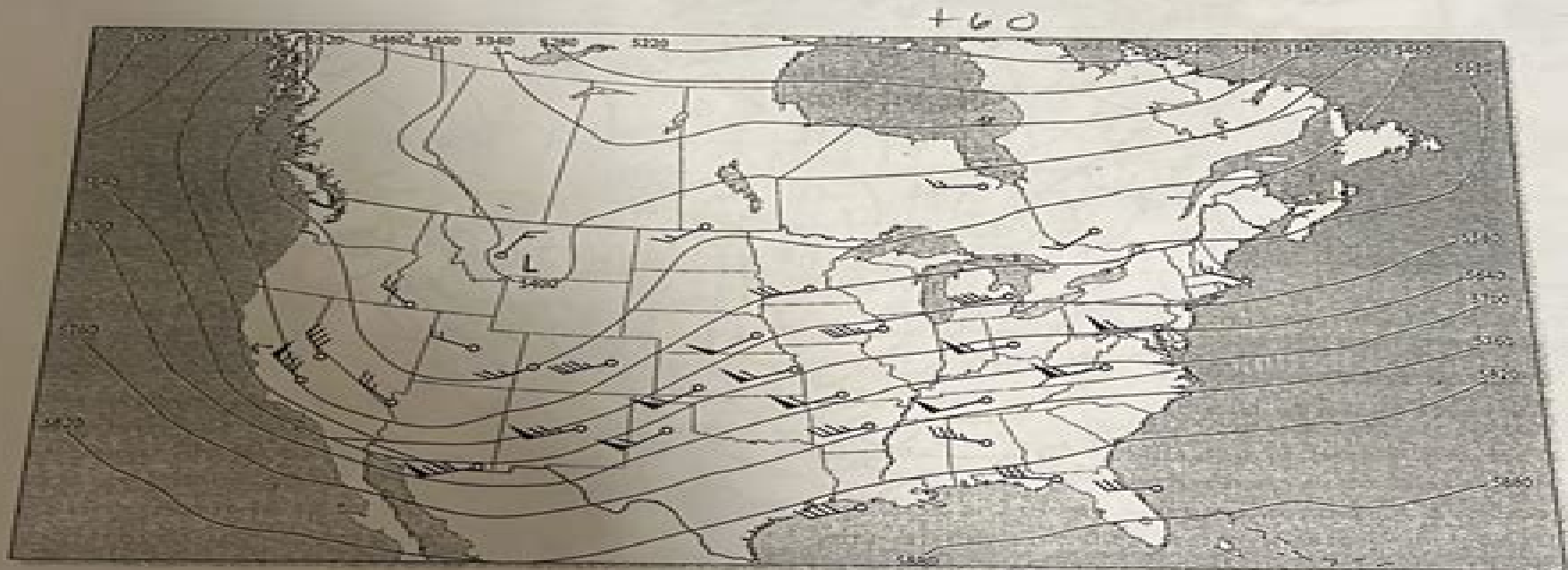
Figure 9-16. A 500-mb map.
