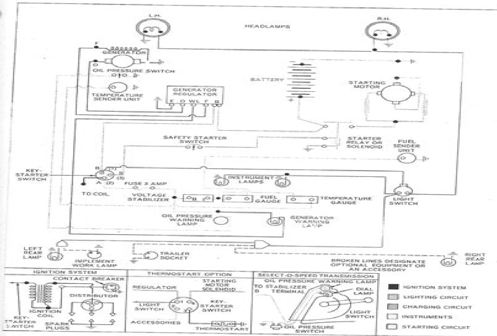
Electrical System Schematic—Tractors with "C" Prefixed Serial Numbers
