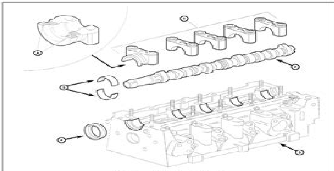
9.28 Camshaft refitting details
