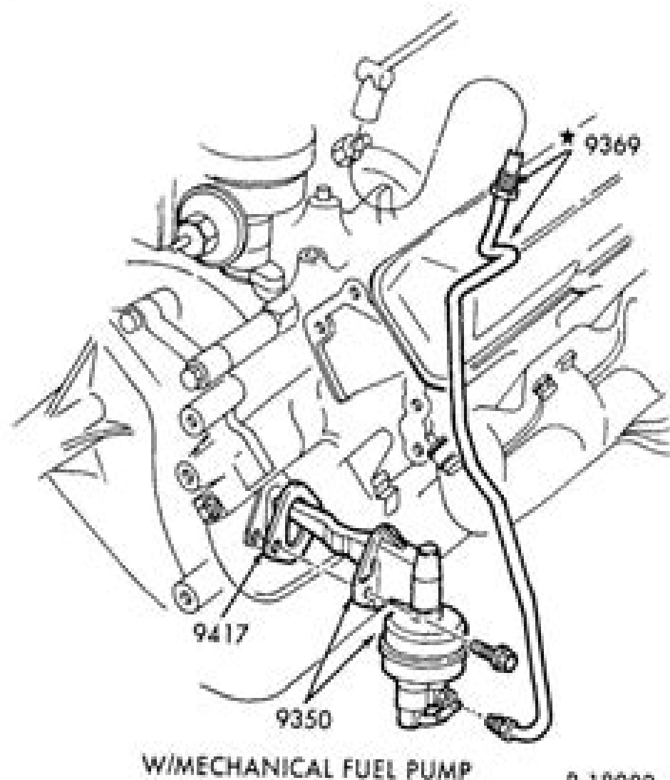
FUEL LINES to CARBURETOR 1983/87 E-F250/350 - 8 CYL. 460 (7.5L)
