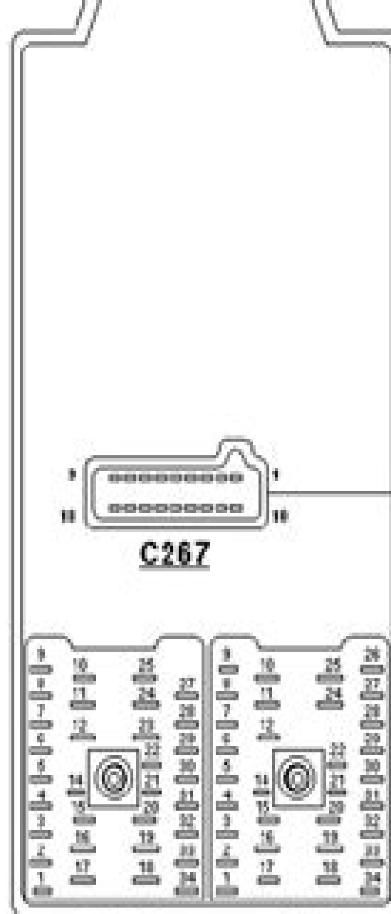
BOTTOM VIEW
