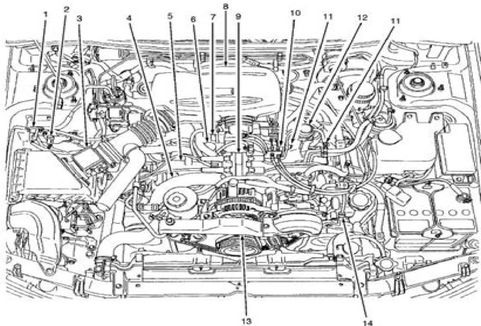
Fig. 3: Component Locations (Legacy 2.5L & Outback 2.5L) SUBARU OF AMERICA, INC.
