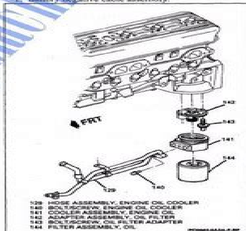
Figure 21 - Engine Oil Cooler and Hose Assembly
