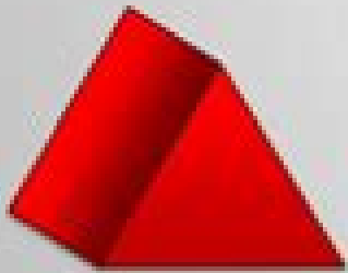
Triangular prism
