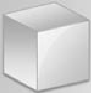
Cube
