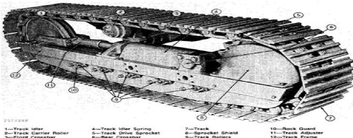
Fig. 1—Track System
