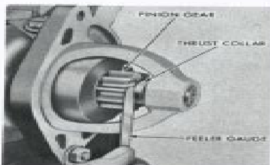
Fig. 133—Measuring starting motor drive pinion clearance. Refer to text for procedure and to Fig. 134 for adjustment of clearance.
