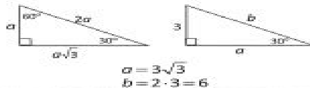
30-60-90 Triangle
