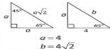
Isosceles Right Triangle
