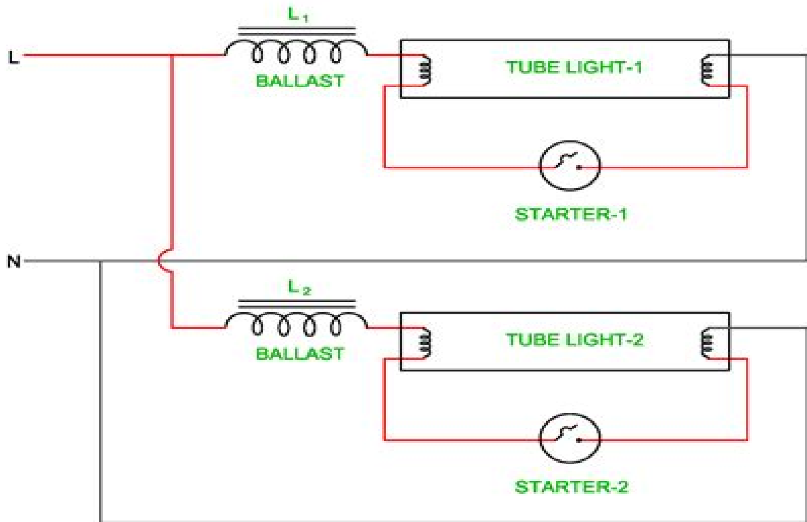
WIRING DIAGRAM OF TWIN TUBE LIGHT
