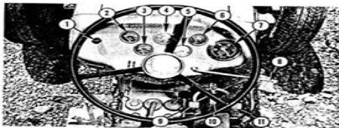
Fig. 2 — Instruments and Controls (Instant Reverse Trans.)
