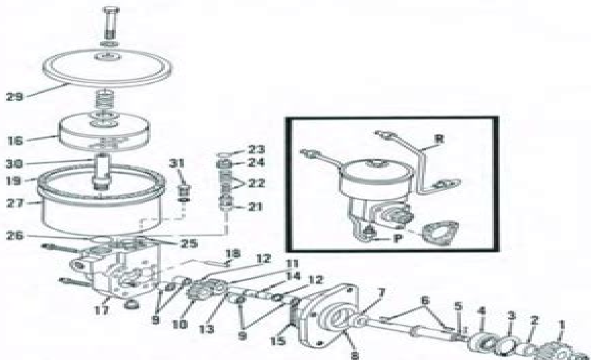
Fig. 11—Exploded view of power steering pump used on Models MF230, MF235 and MF245 equipped with gasoline engine. Inset shows location of pressure line (P) and return line (R).
