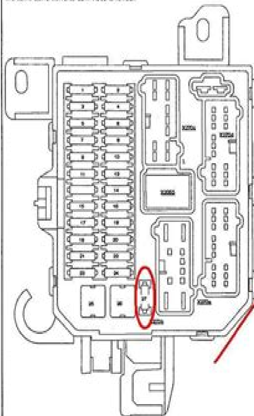
K-070a DASH PANEL HEADLAMP JUMPER
