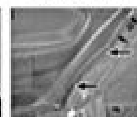
1.29 Unscrew the bolts (arrowed) at the base of the panel
