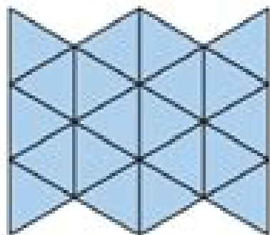
Regular tessellation
