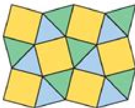
Semiregular tessellation
