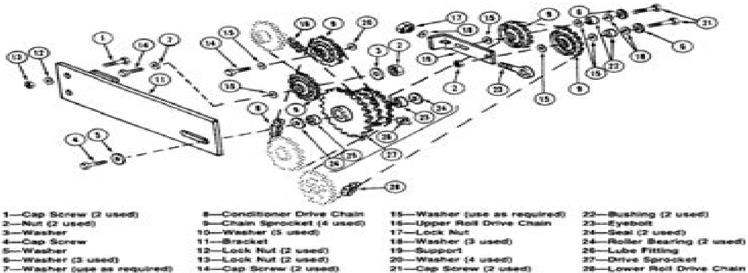
Exploded View of Conditioner Drives
