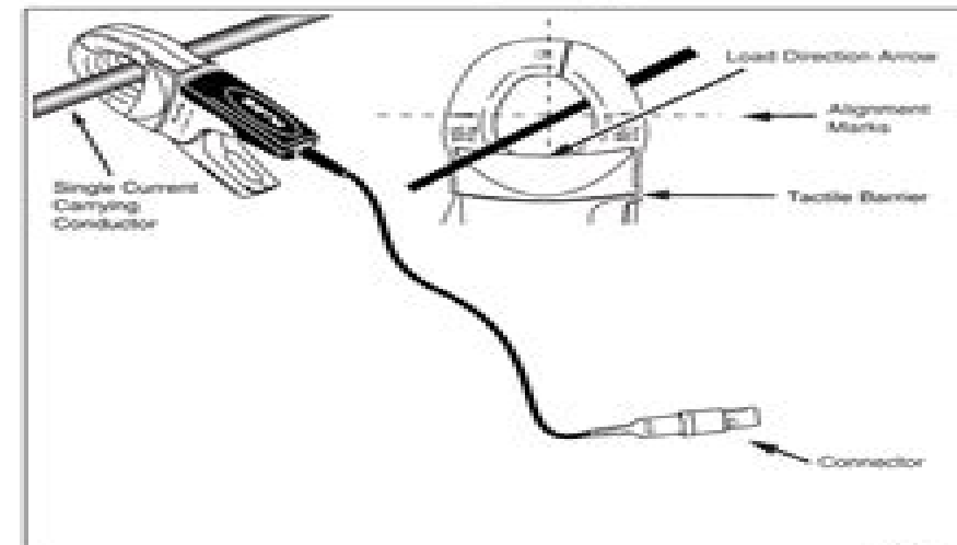
Figure 1.3140R Setup
